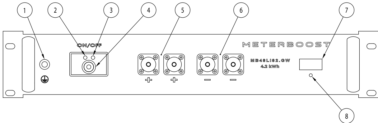
Figure 1: Battery front.
