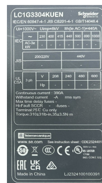
Schneider LC1G3304KUEN contactor
